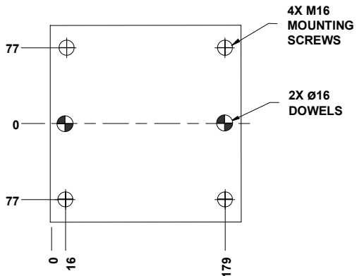
BOTTOM VIEW (Driver Only)
