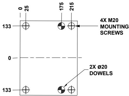
TOP VIEW (Driver Only)
