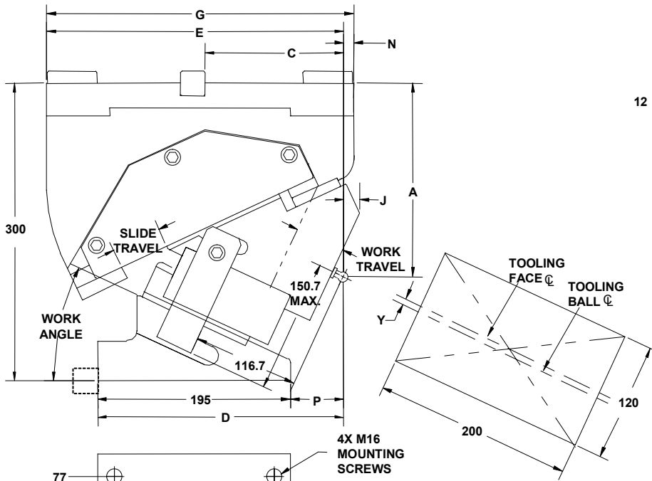
TOOLING MOUNTING FACE
